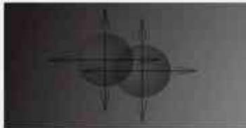
A photon is split into two entangled photons.
