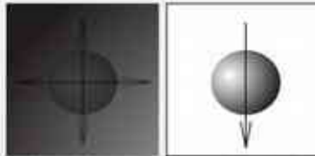
Unobserved photon exists in all possible states.
